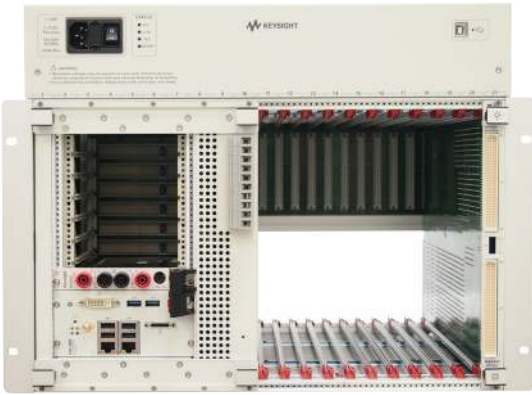
Figure 1. U8989A – front
